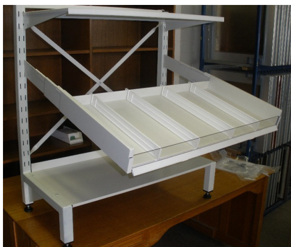
Photos showing a sloping open view tray in its normal position and in an extended position for easy loading.
